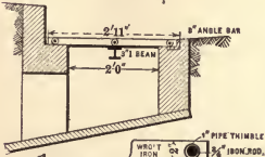
FIG. 1. FLUSHTANK
